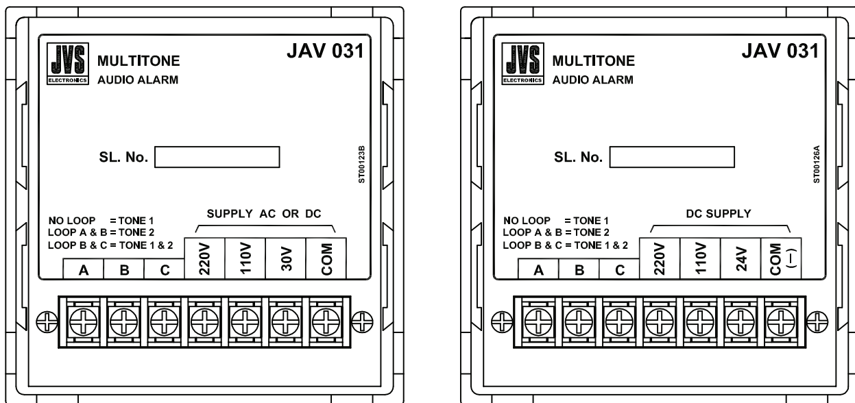
REAR VIEW OF RELAY SHOWING TERMINAL ARRANGEMENT
